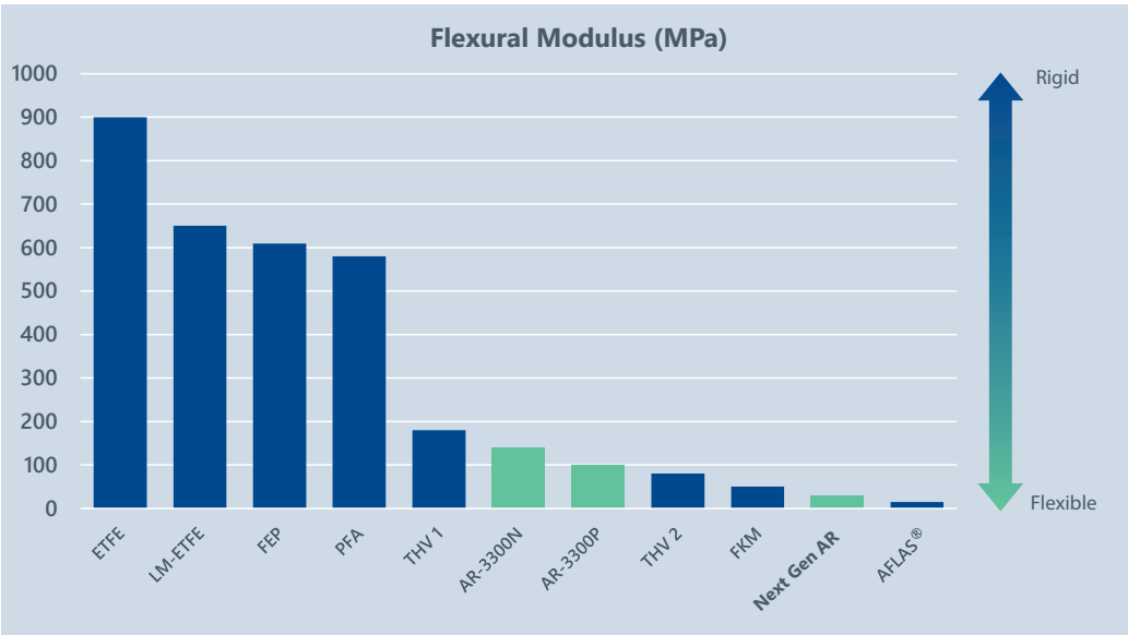
Fluon+™ AR-ETFE flexibility comparison with other common fluoropolymers and fluoroelastomers
