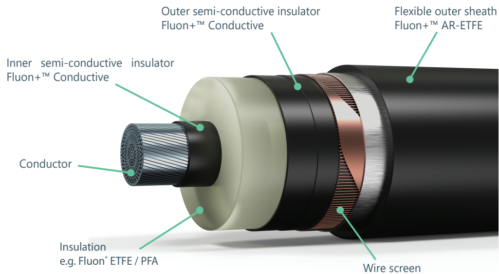
Illustration of where Fluon+™ and Fluon® products can be used within a high voltage cable
